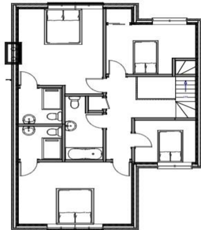
PROPOSED 1ST FLOOR PLAN SCALE 1:50
