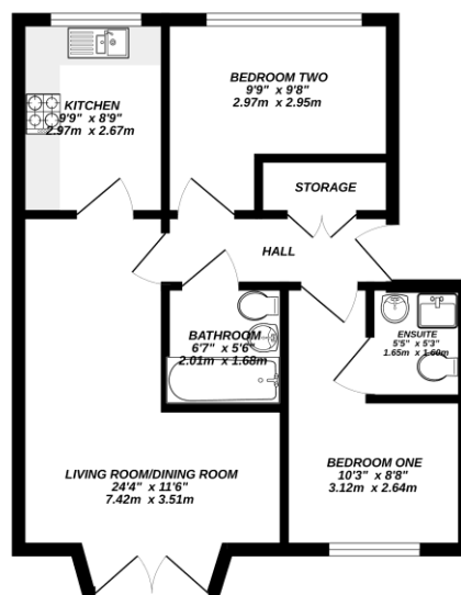
SECOND FLOOR
